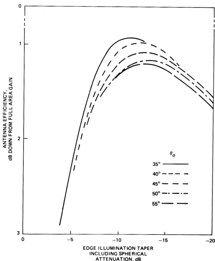
Fig. 4—Antenna efficiency as a function of edge illumination for various values of subtended dish half-angle, \theta_o .
